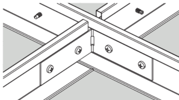
DETAIL B - CROSS TEE ADAPTER CLIP
