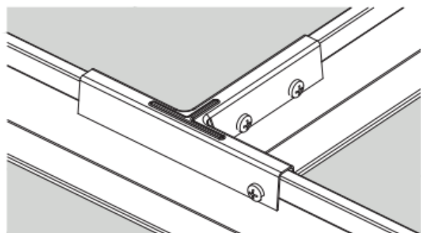
DETAIL A - CONNECTOR DB3
